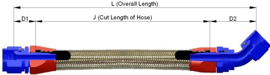
Assembly length with double swivel hose ends fitting (1000 series)
